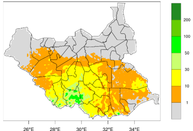
Rainfall Forecast (mm): 05 Mar-12 Mar 2024
