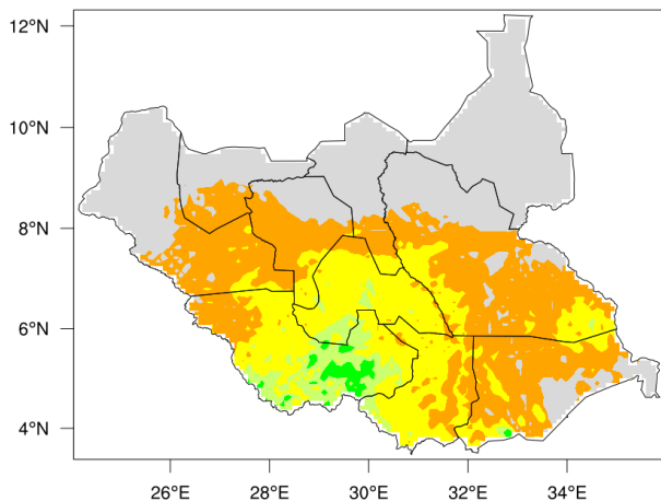
Rainfall Forecast (mm): 05 Mar-12 Mar 2024
