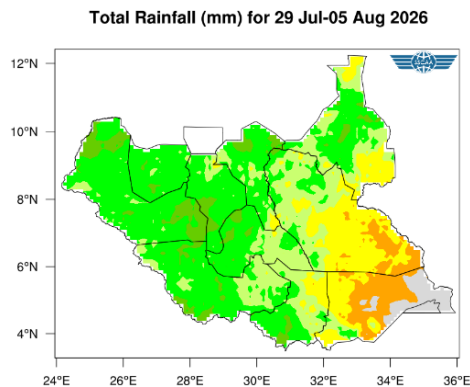
Figure 2a: Total rainfall(mm) forecast for 29 July to 05 Aug 2026
