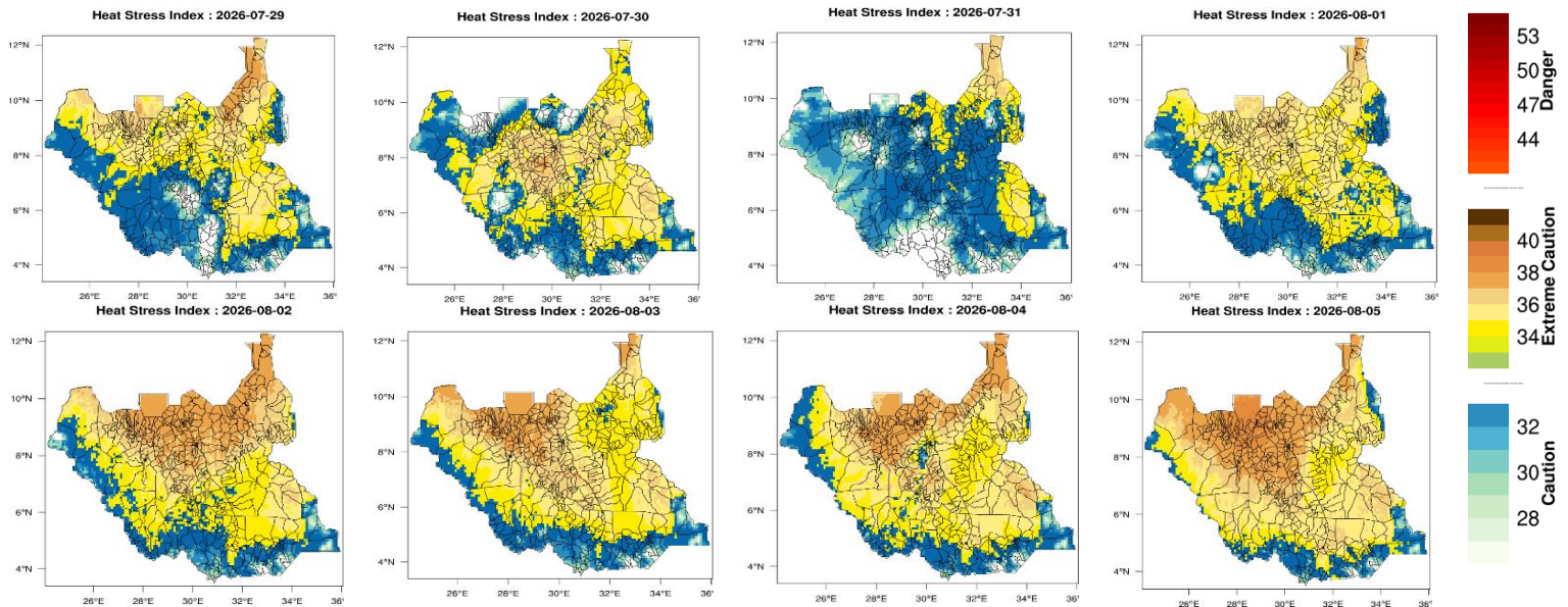
Figure 5: Heat Stress Index forecast for 29 July to 05 Aug 2026
