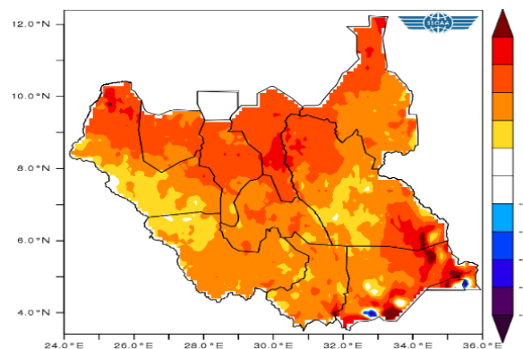
Figure 3b: Temp. Anomalies (°C) forecast for 28/7-04/8 2026
