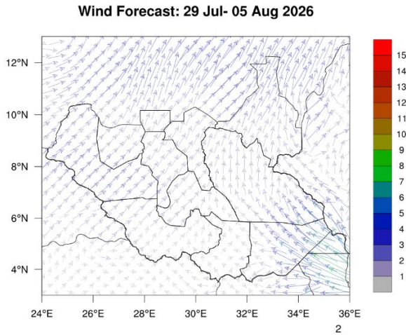
Figure 4: Wind (Direction & Speed) forecast for 29/7-05/8 2026
