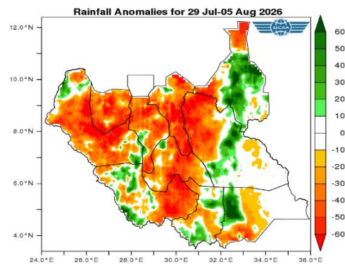
Figure 2b: Rainfall anomalies 29 July to 05 Aug 2026
